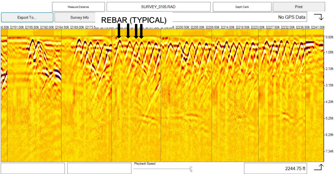
Image Set 4. Rebar in eastern survey area
