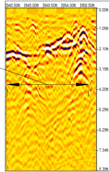
GROUND PENETRATION RADAR 8FT X 20 FT NATIVE SOILS DISTURBED
