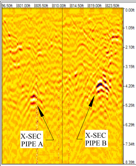
GROUND PENETRATION RADAR PIPE A & B
