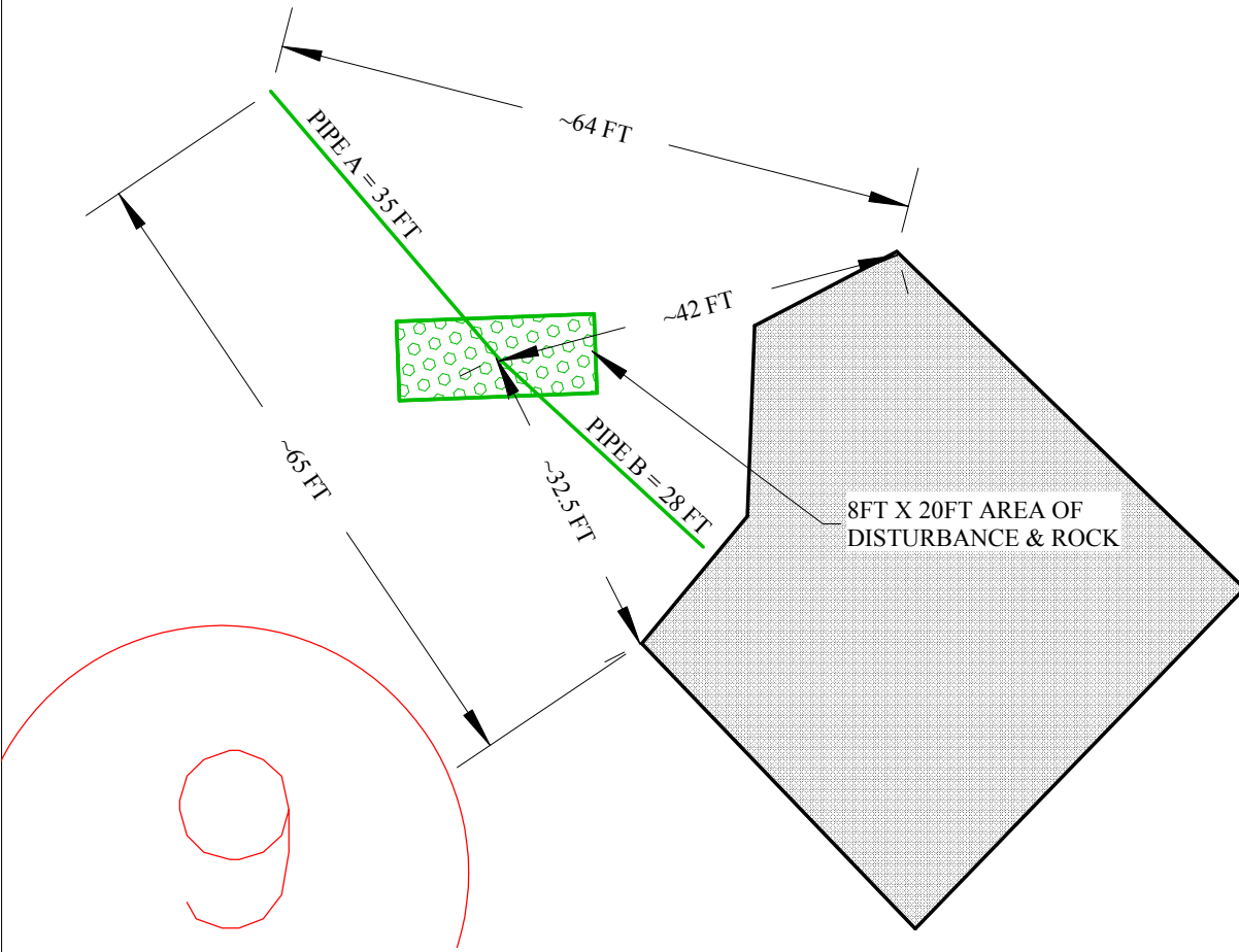
GROUND PENETRATION RADAR 8FT X 20 FT NATIVE SOILS DISTURBED
