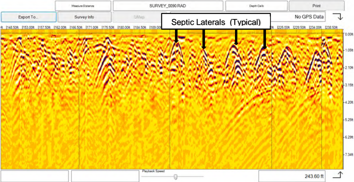
Picture 1. Orientation of septic laterals. For visual reference only.
